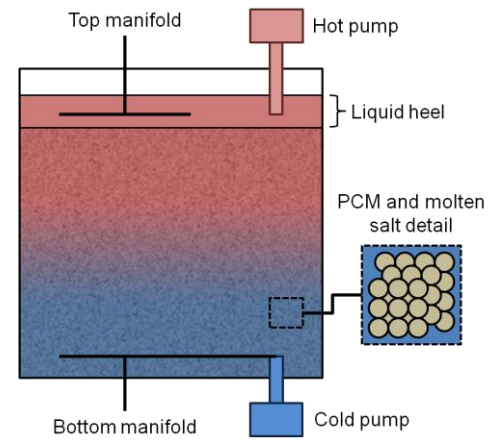
Illustration of thermocline tank with PCM
